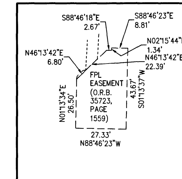
FPL EASEMENT DETAIL
